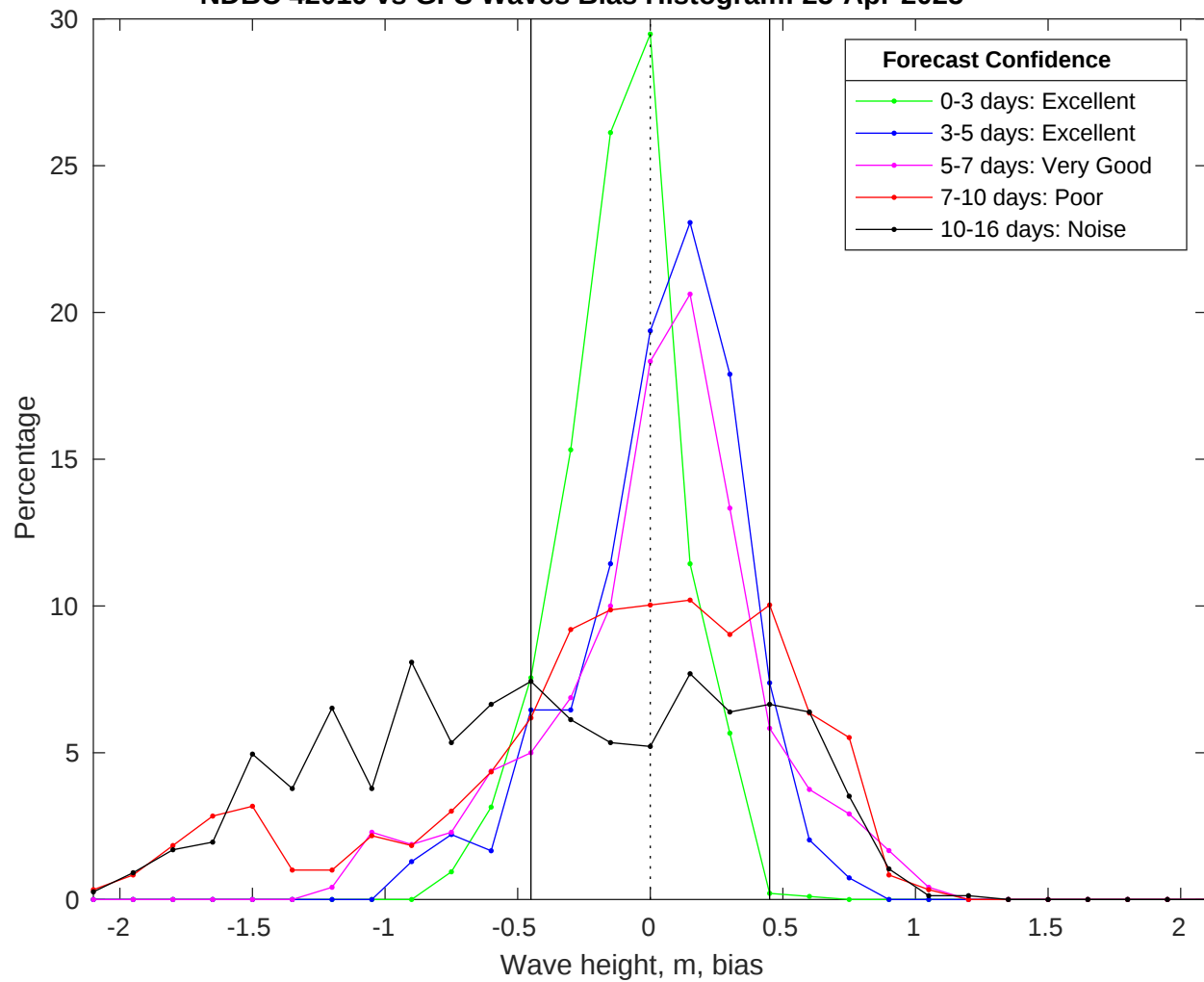
NDBC 42019 vs GFS Waves Bias Histogram: 25-Apr-2025
