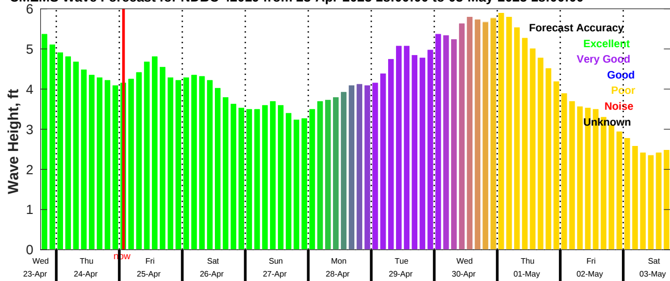
CMEMS Wave Forecast for NDBC 42019 from 23-Apr-2025 18:00:00 to 03-May-2025 18:00:00
