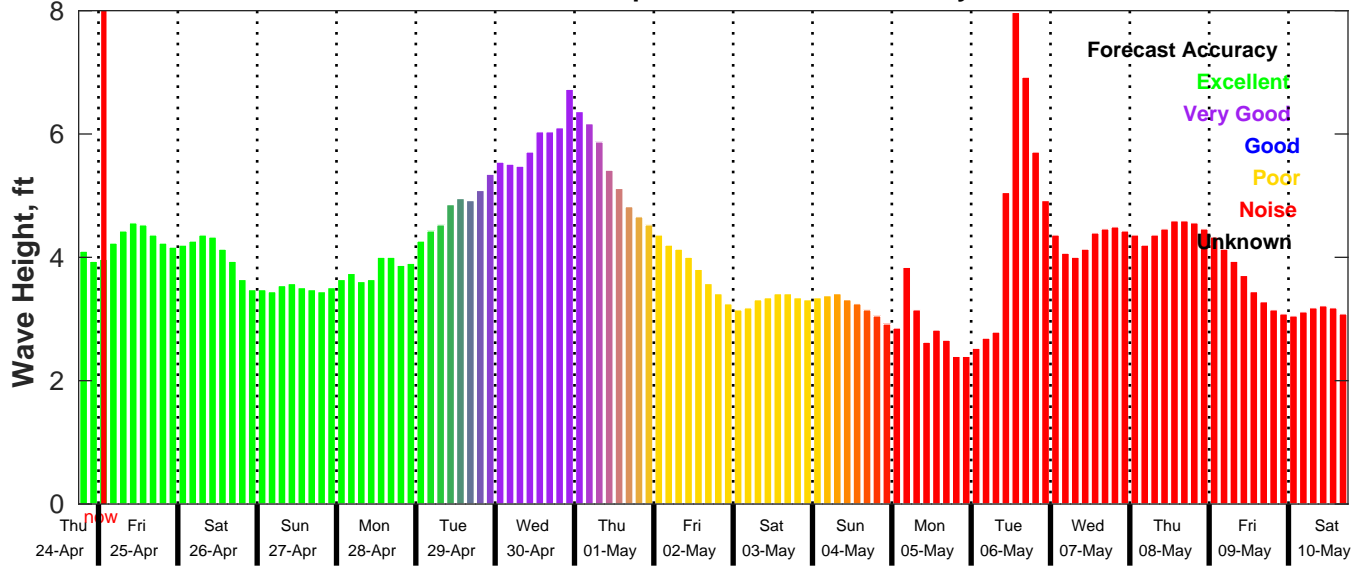
GFS Wave Forecast for NDBC 42019 from 24-Apr-2025 18:00:00 to 10-May-2025 18:00:00
