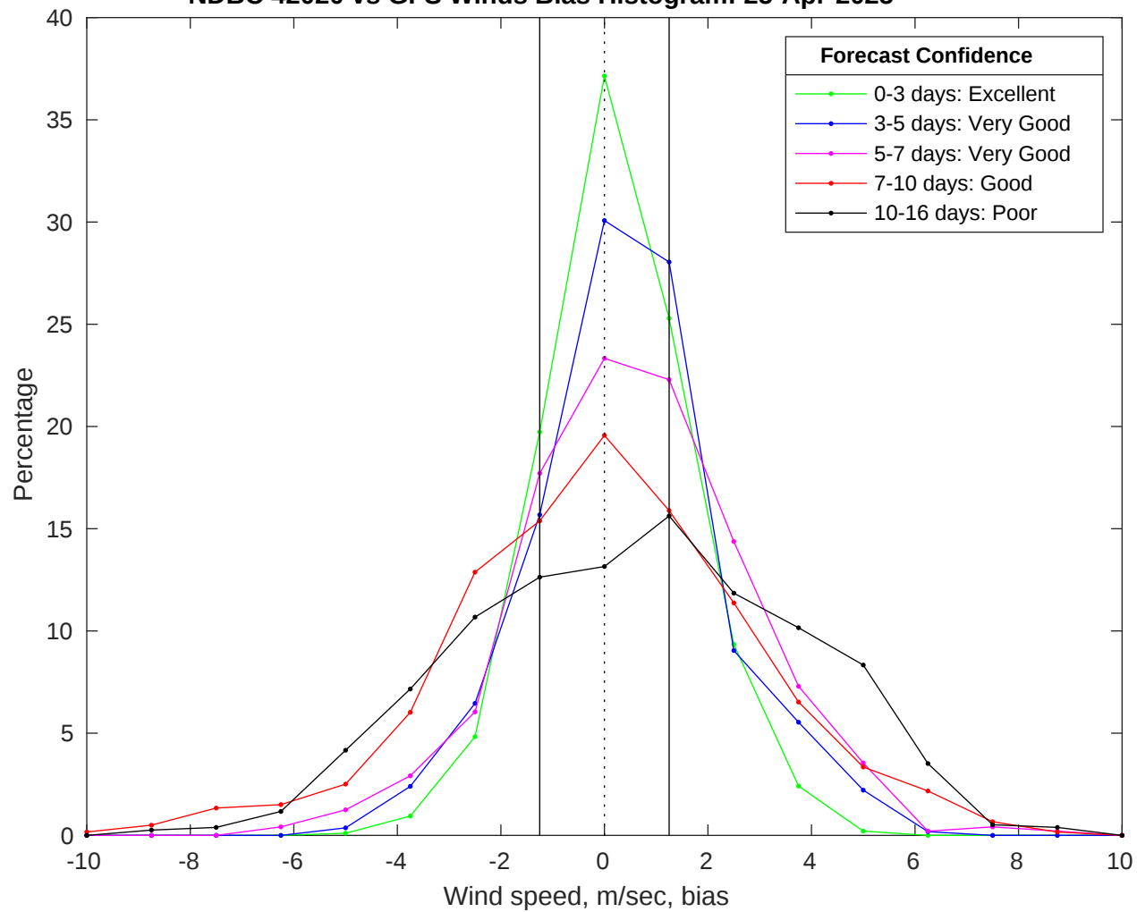
NDBC 42020 vs GFS Winds Bias Histogram: 25-Apr-2025
