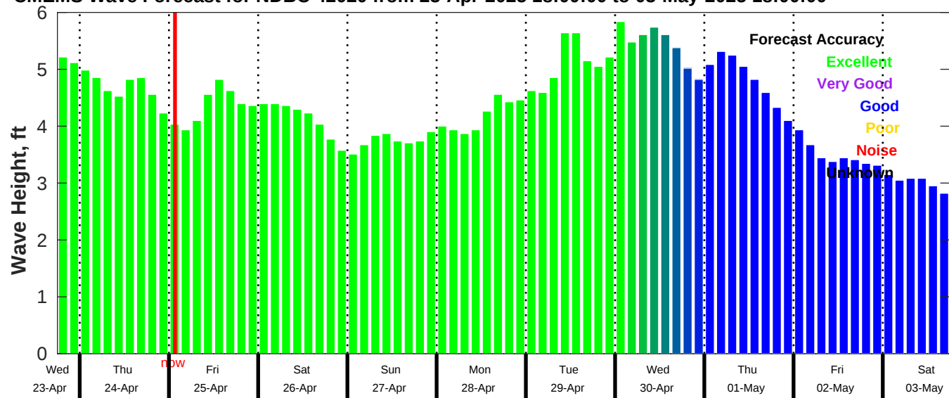
CMEMS Wave Forecast for NDBC 42020 from 23-Apr-2025 18:00:00 to 03-May-2025 18:00:00
