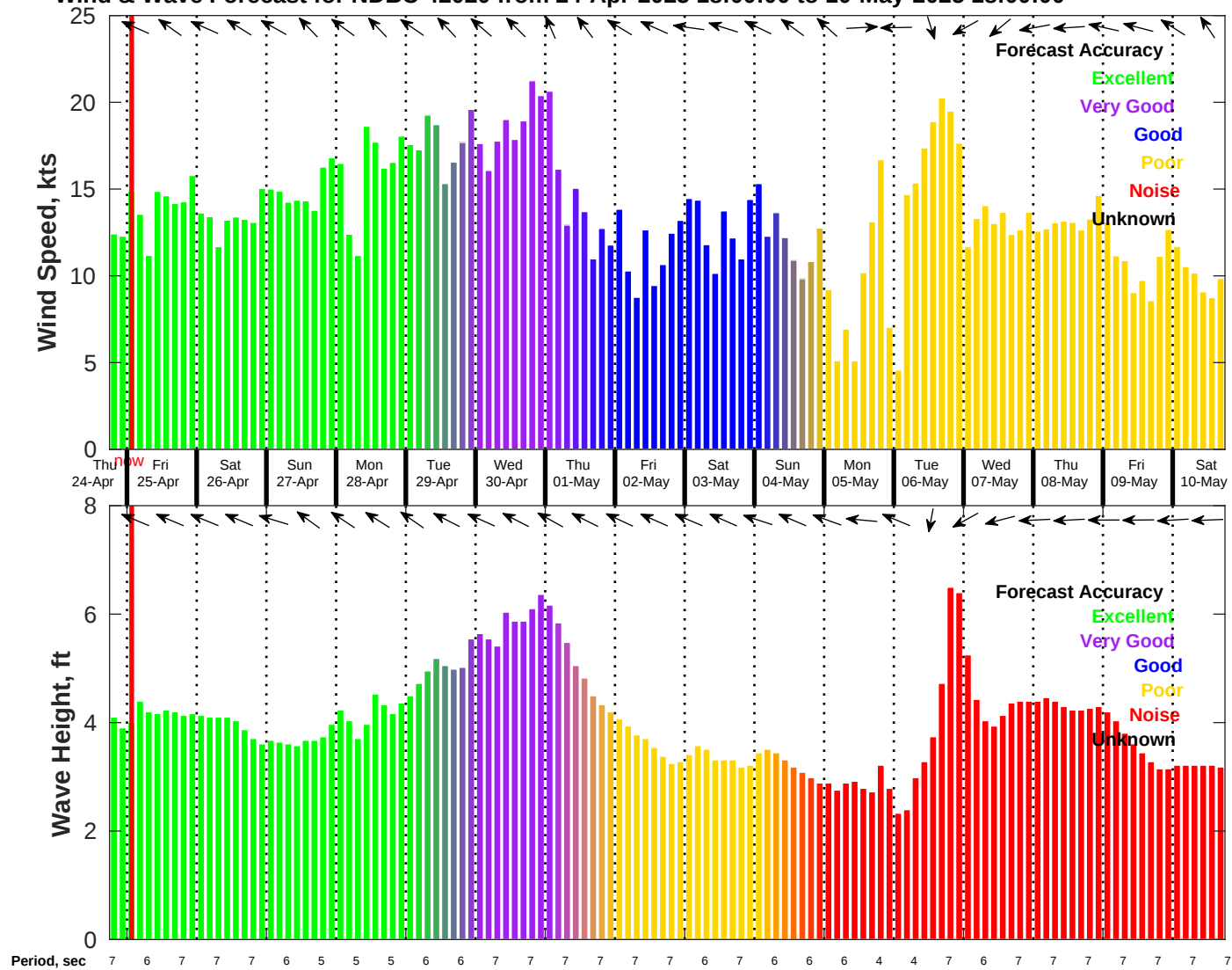
Wind & Wave Forecast for NDBC 42020 from 24-Apr-2025 18:00:00 to 10-May-2025 18:00:00
