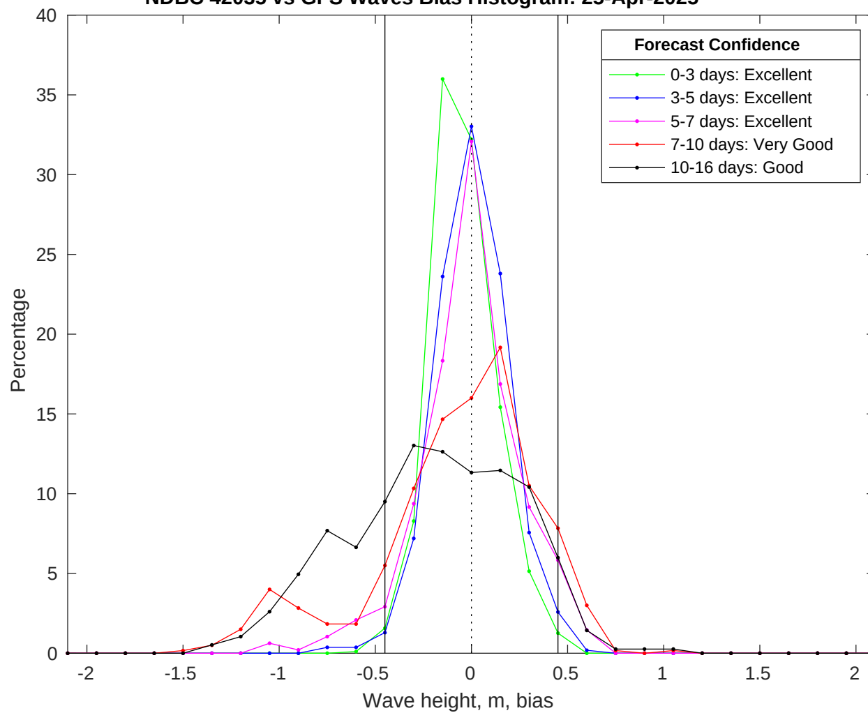
NDBC 42035 vs GFS Waves Bias Histogram: 25-Apr-2025
