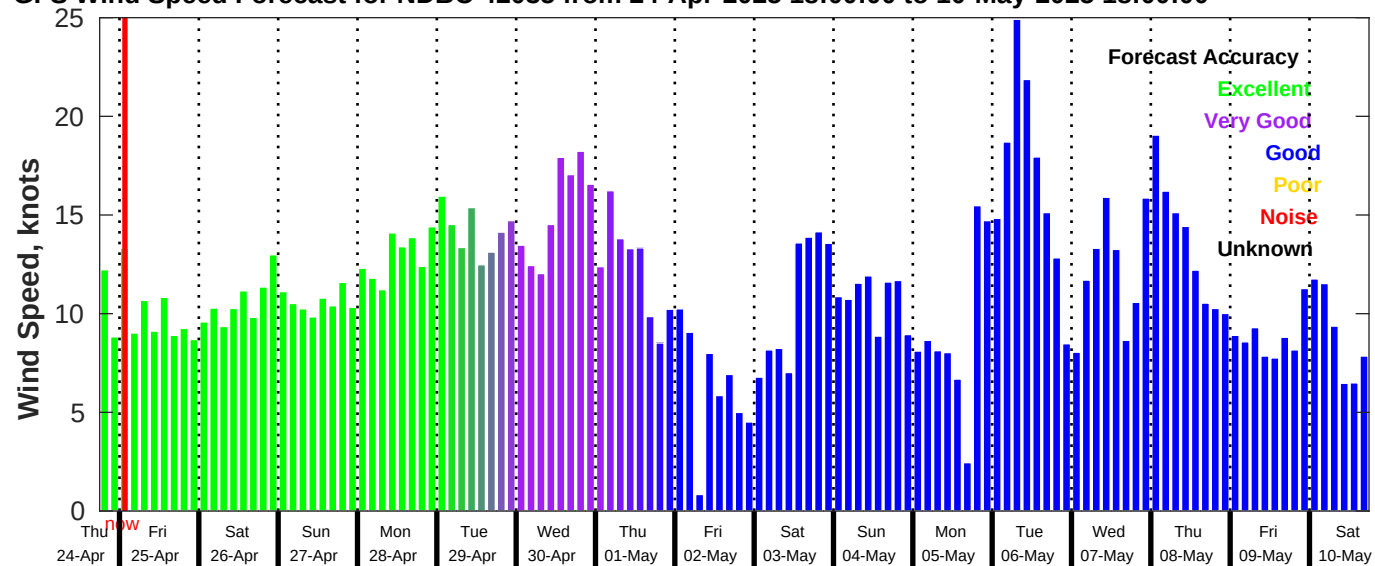
GFS Wind Speed Forecast for NDBC 42035 from 24-Apr-2025 18:00:00 to 10-May-2025 18:00:00
