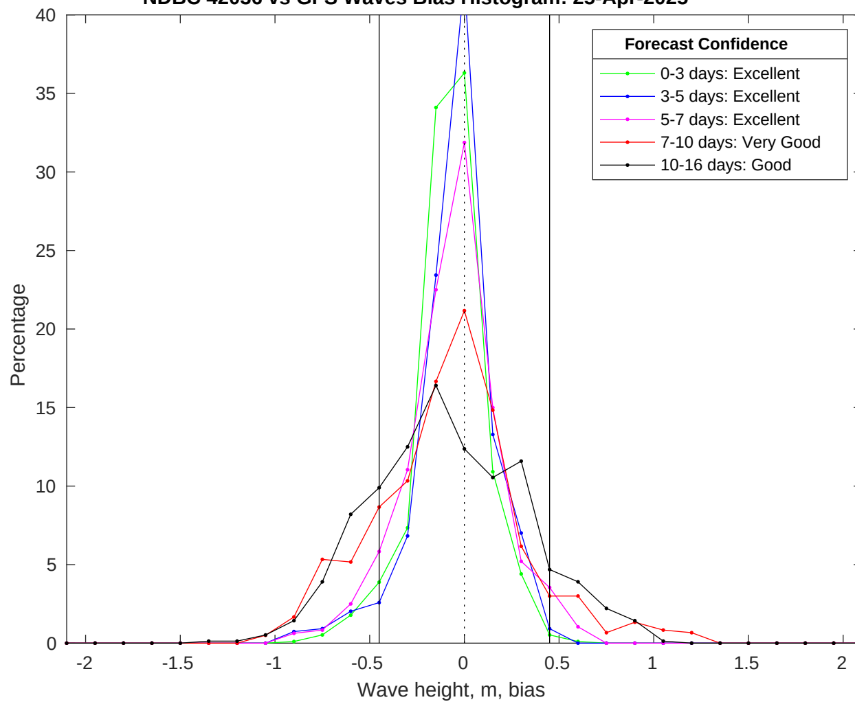
NDBC 42036 vs GFS Waves Bias Histogram: 25-Apr-2025
