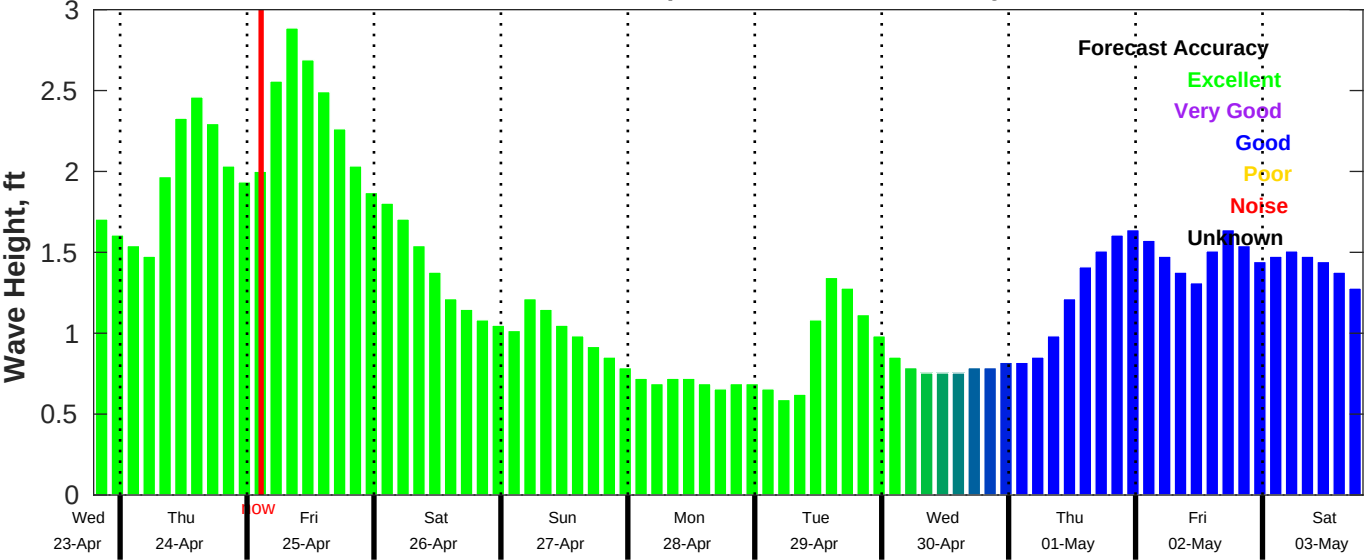
CMEMS Wave Forecast for NDBC 42036 from 23-Apr-2025 19:00:00 to 03-May-2025 19:00:00
