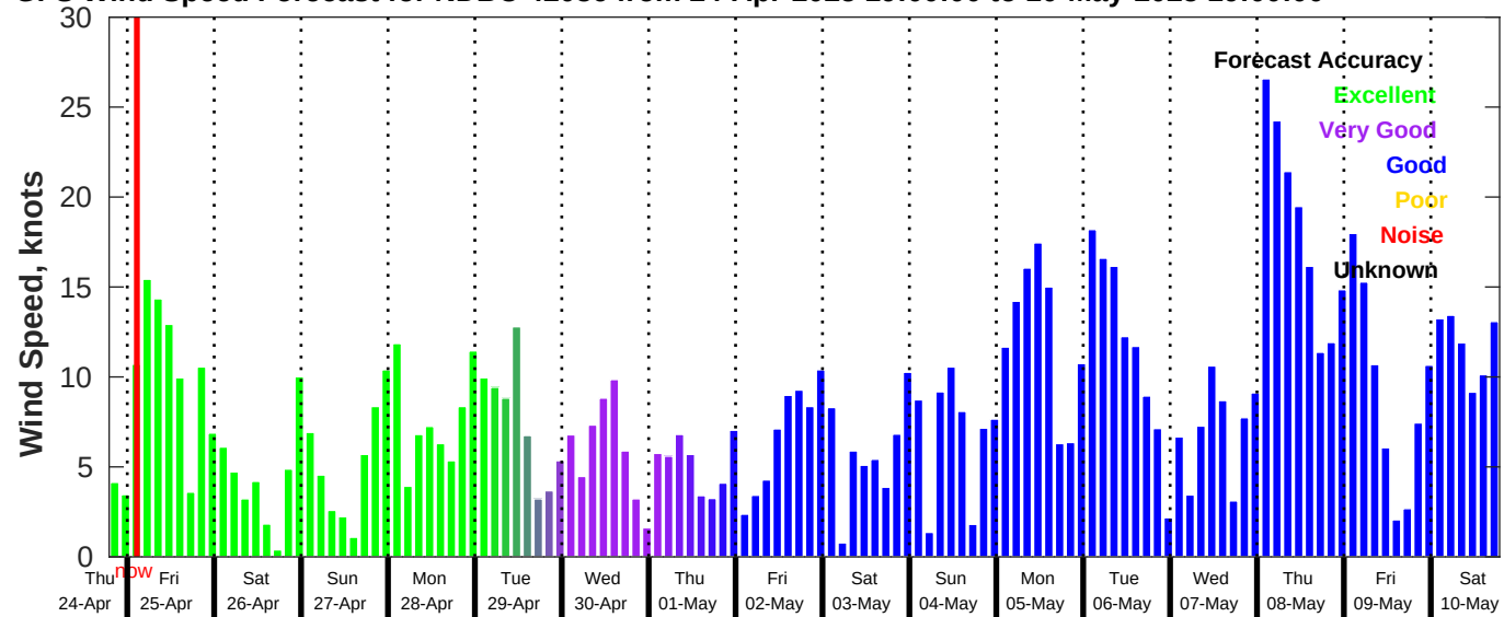
GFS Wind Speed Forecast for NDBC 42036 from 24-Apr-2025 19:00:00 to 10-May-2025 19:00:00
