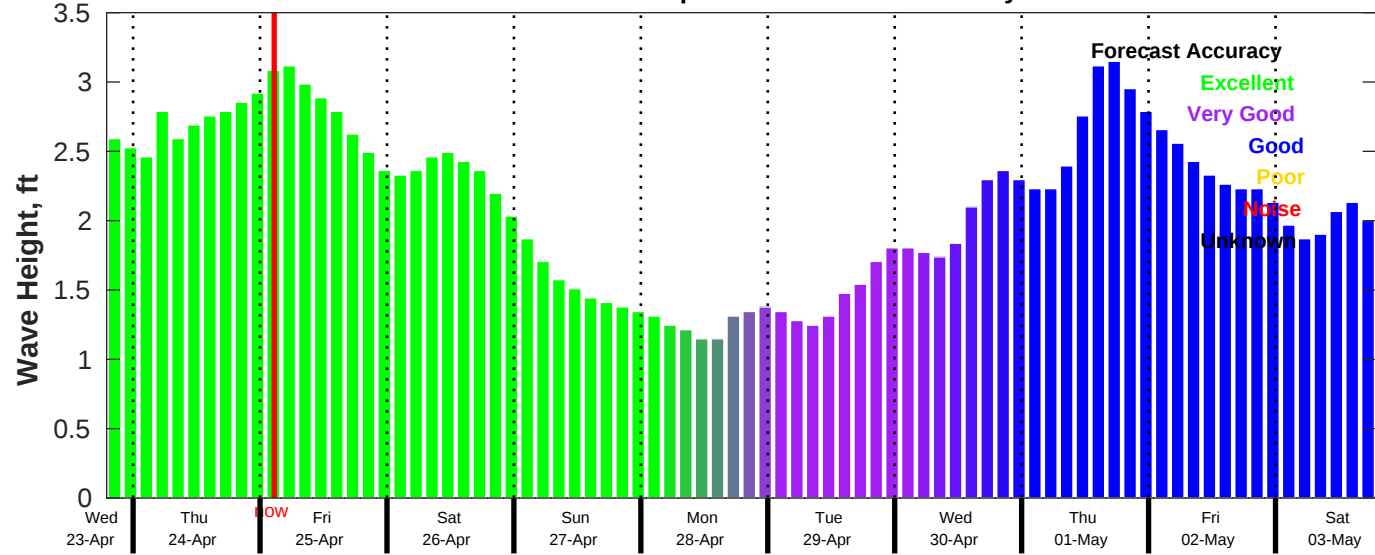
CMEMS Wave Forecast for NDBC 42040 from 23-Apr-2025 19:00:00 to 03-May-2025 19:00:00
