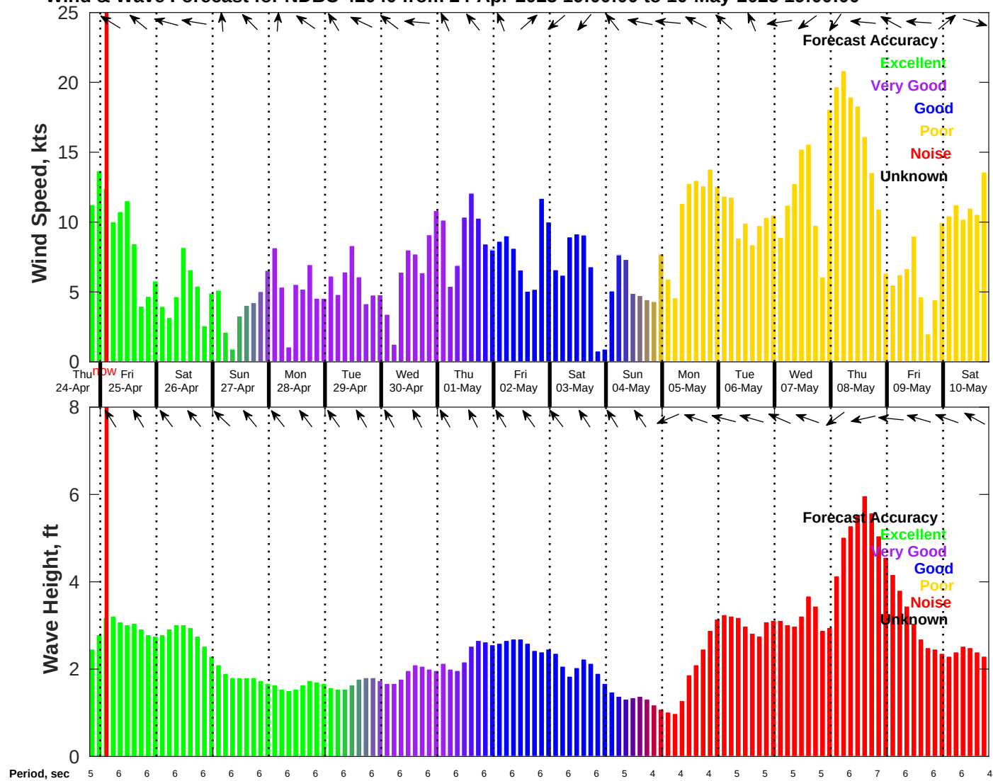
Wind & Wave Forecast for NDBC 42040 from 24-Apr-2025 19:00:00 to 10-May-2025 19:00:00
