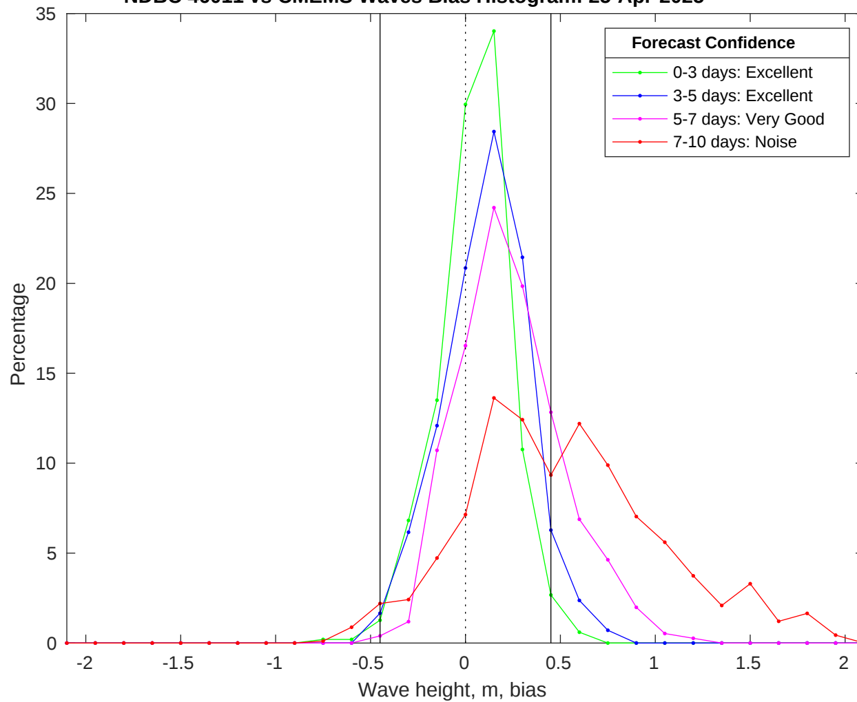
NDBC 46011 vs CMEMS Waves Bias Histogram: 25-Apr-2025
