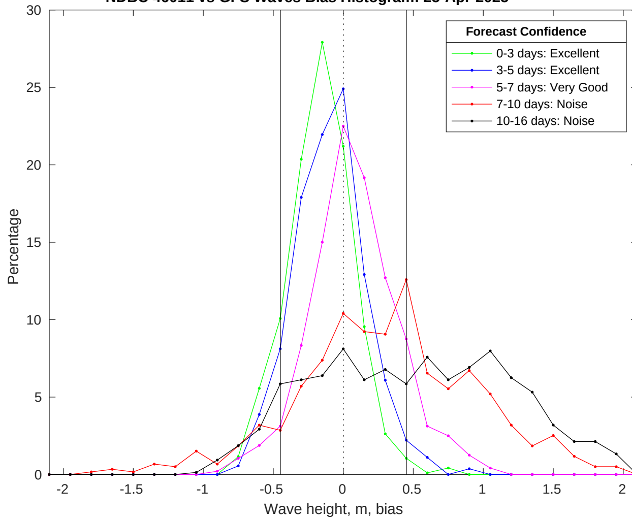
NDBC 46011 vs GFS Waves Bias Histogram: 25-Apr-2025
