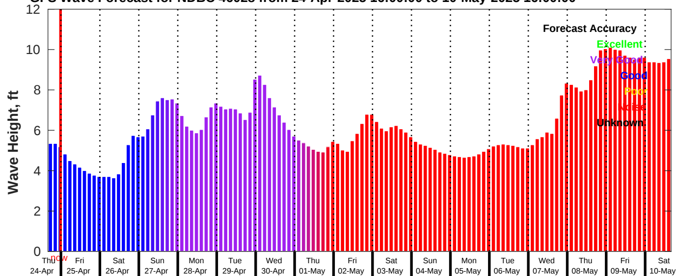
GFS Wave Forecast for NDBC 46028 from 24-Apr-2025 16:00:00 to 10-May-2025 16:00:00
