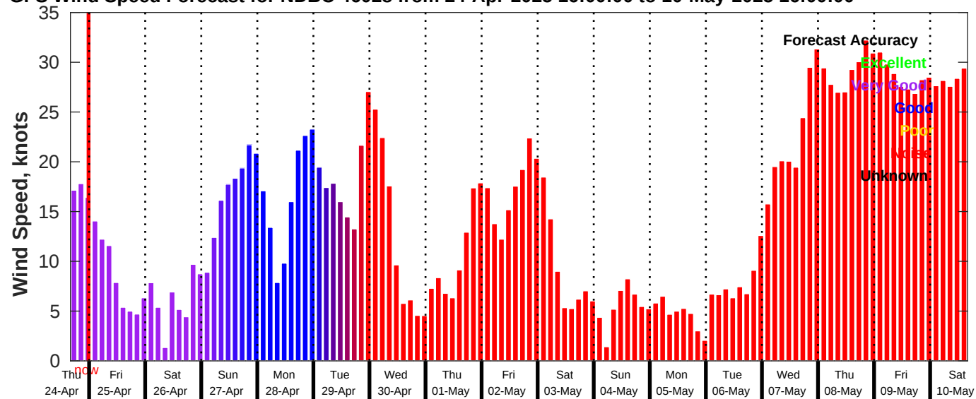
GFS Wind Speed Forecast for NDBC 46028 from 24-Apr-2025 16:00:00 to 10-May-2025 16:00:00
