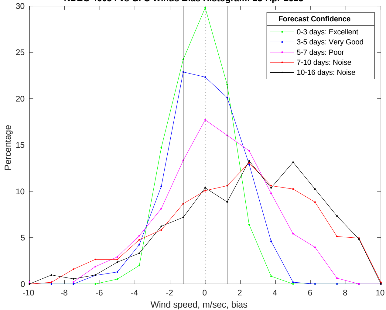
NDBC 46054 vs GFS Winds Bias Histogram: 25-Apr-2025
