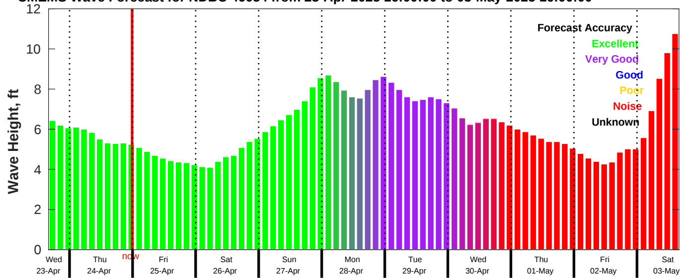
CMEMS Wave Forecast for NDBC 46054 from 23-Apr-2025 16:00:00 to 03-May-2025 16:00:00
