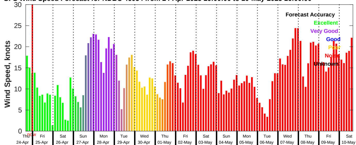
GFS Wind Speed Forecast for NDBC 46054 from 24-Apr-2025 16:00:00 to 10-May-2025 16:00:00
