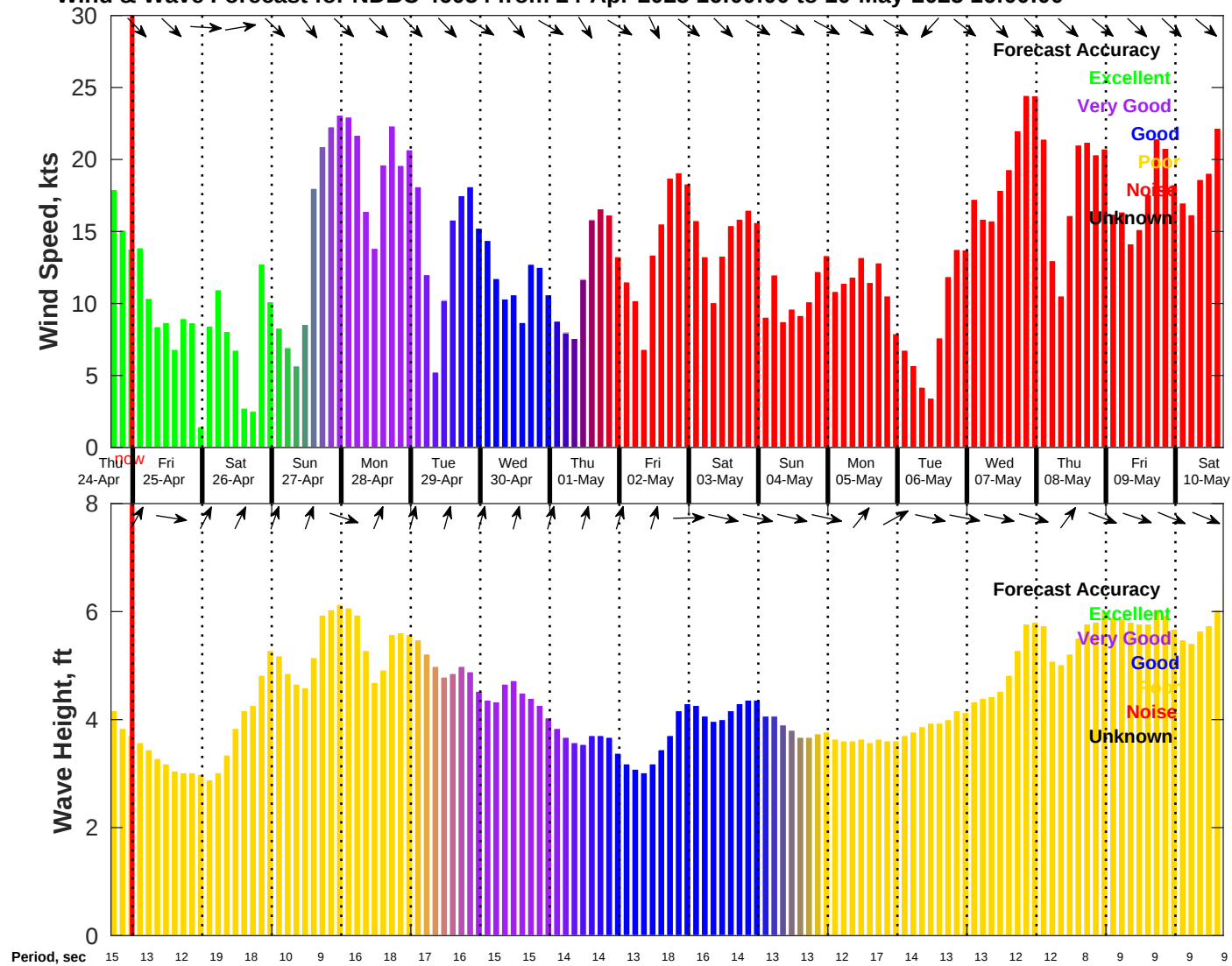
Wind & Wave Forecast for NDBC 46054 from 24-Apr-2025 16:00:00 to 10-May-2025 16:00:00
