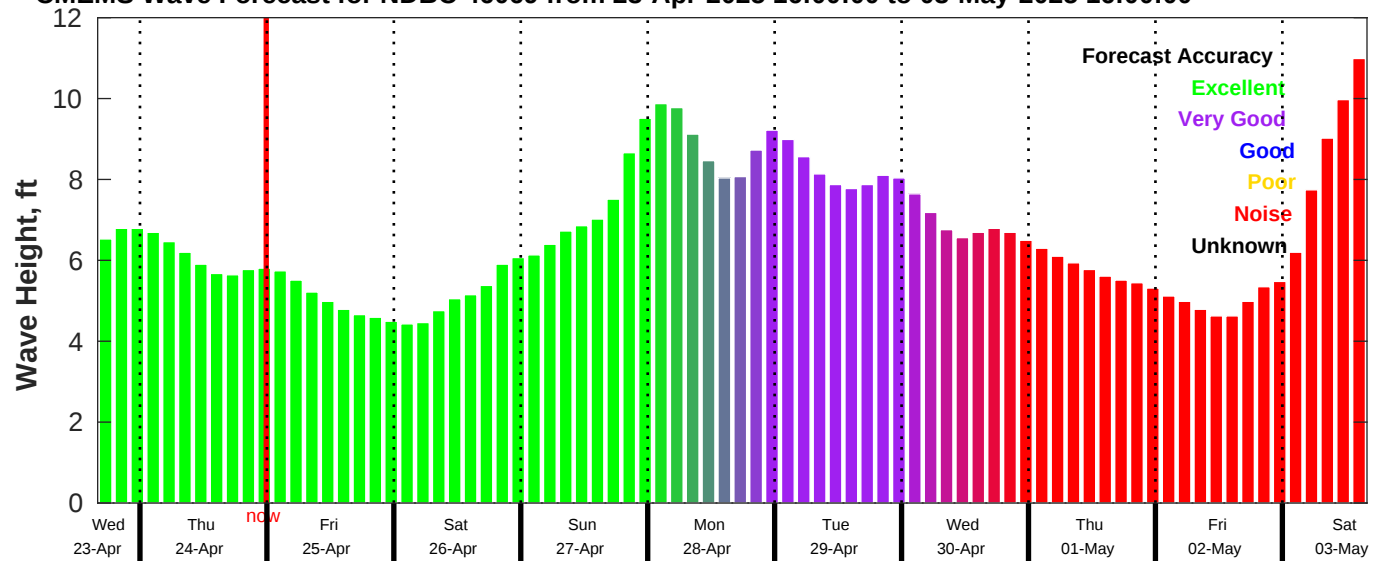
CMEMS Wave Forecast for NDBC 46069 from 23-Apr-2025 16:00:00 to 03-May-2025 16:00:00
