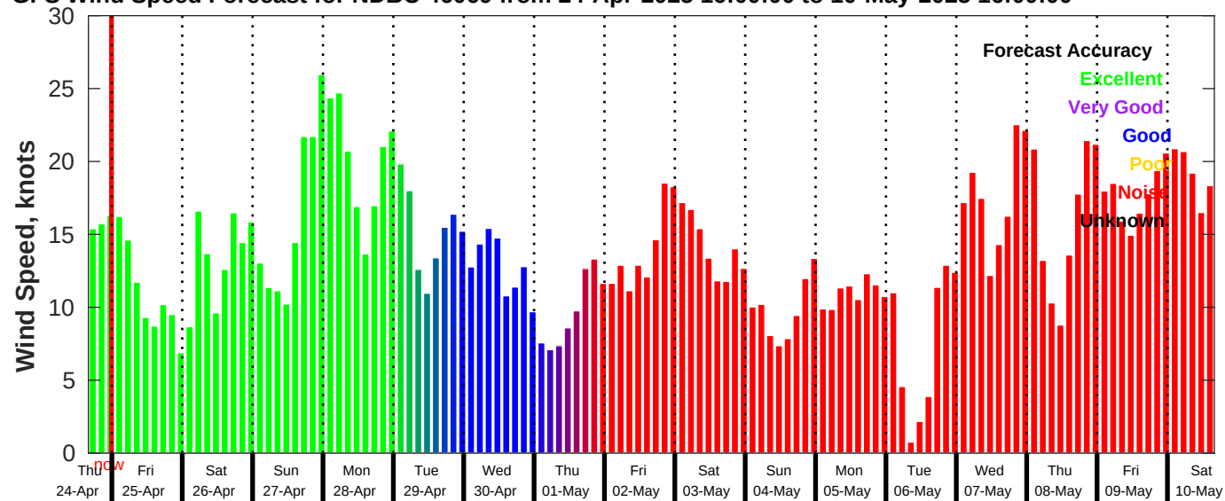
GFS Wind Speed Forecast for NDBC 46069 from 24-Apr-2025 16:00:00 to 10-May-2025 16:00:00
