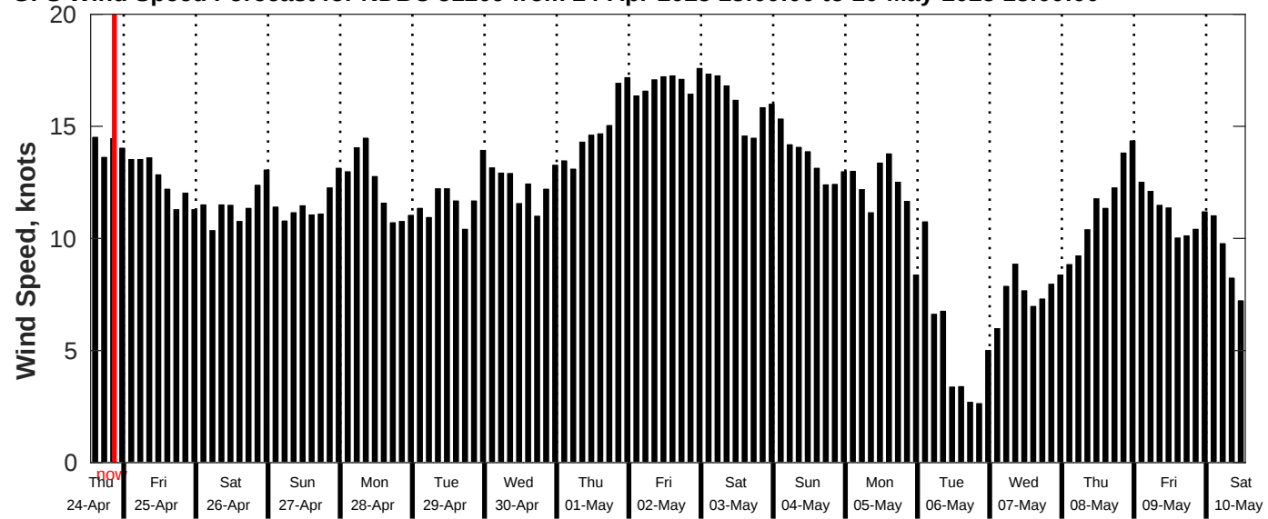
GFS Wind Speed Forecast for NDBC 51209 from 24-Apr-2025 13:00:00 to 10-May-2025 13:00:00
