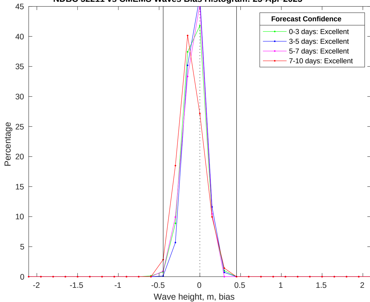
NDBC 52211 vs CMEMS Waves Bias Histogram: 25-Apr-2025
