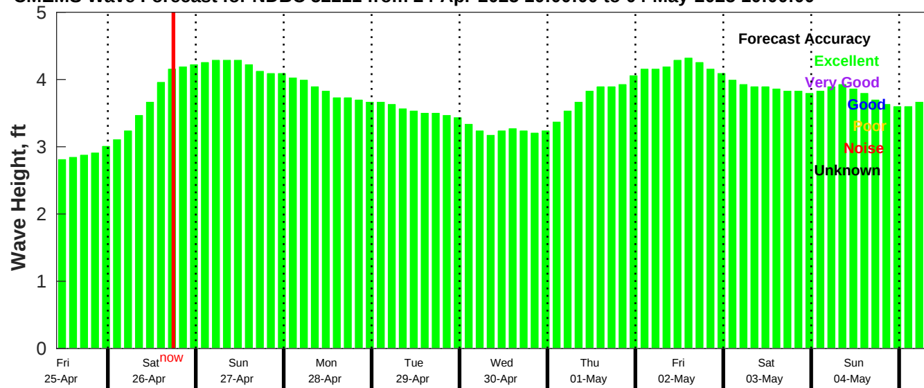
CMEMS Wave Forecast for NDBC 52211 from 24-Apr-2025 10:00:00 to 04-May-2025 10:00:00
