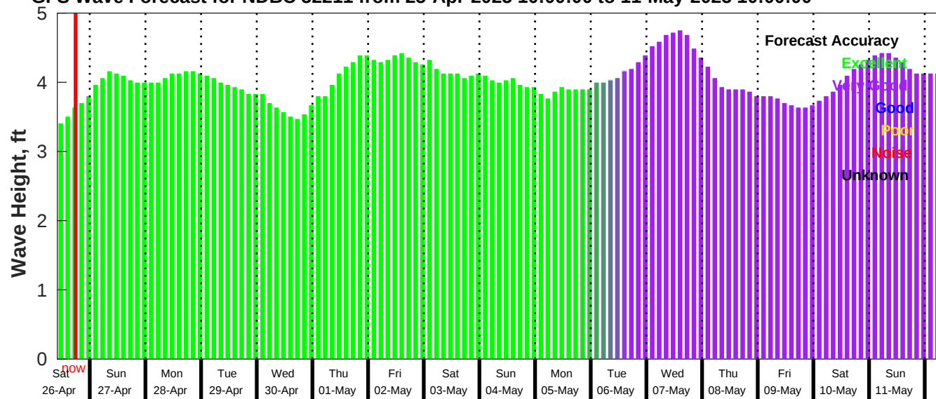
GFS Wave Forecast for NDBC 52211 from 25-Apr-2025 10:00:00 to 11-May-2025 10:00:00
