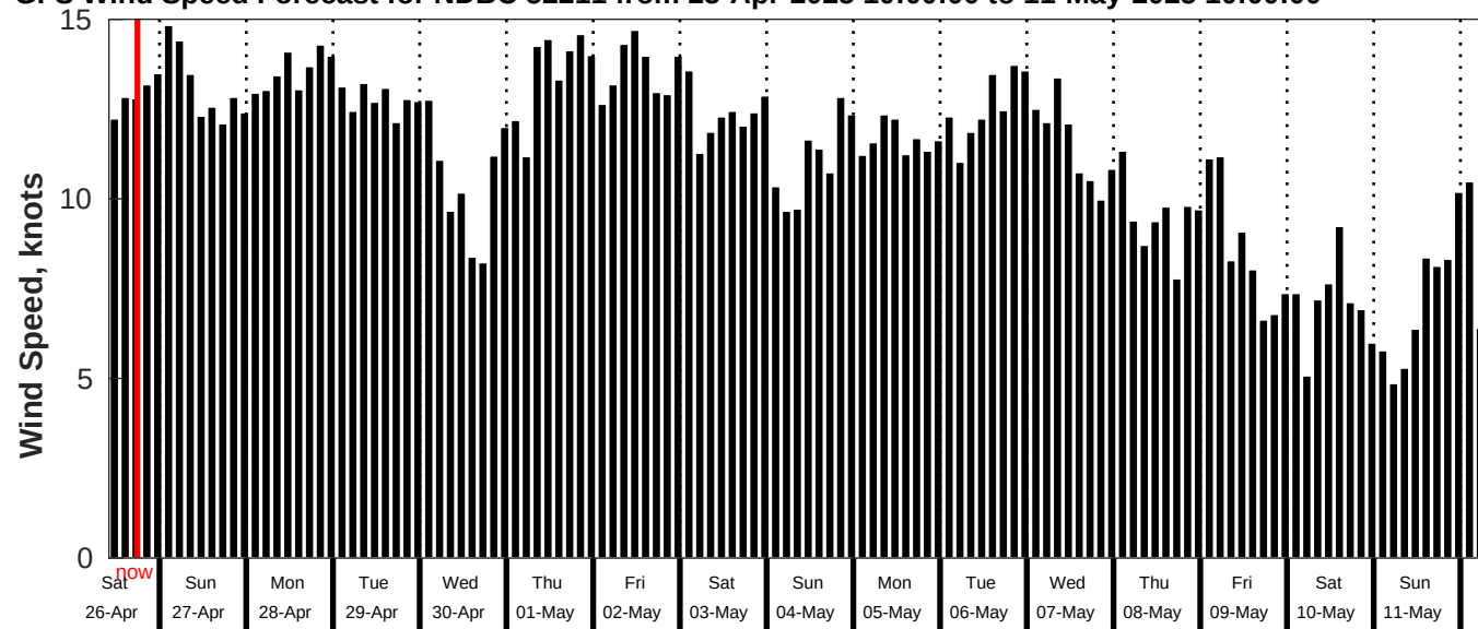
GFS Wind Speed Forecast for NDBC 52211 from 25-Apr-2025 10:00:00 to 11-May-2025 10:00:00
