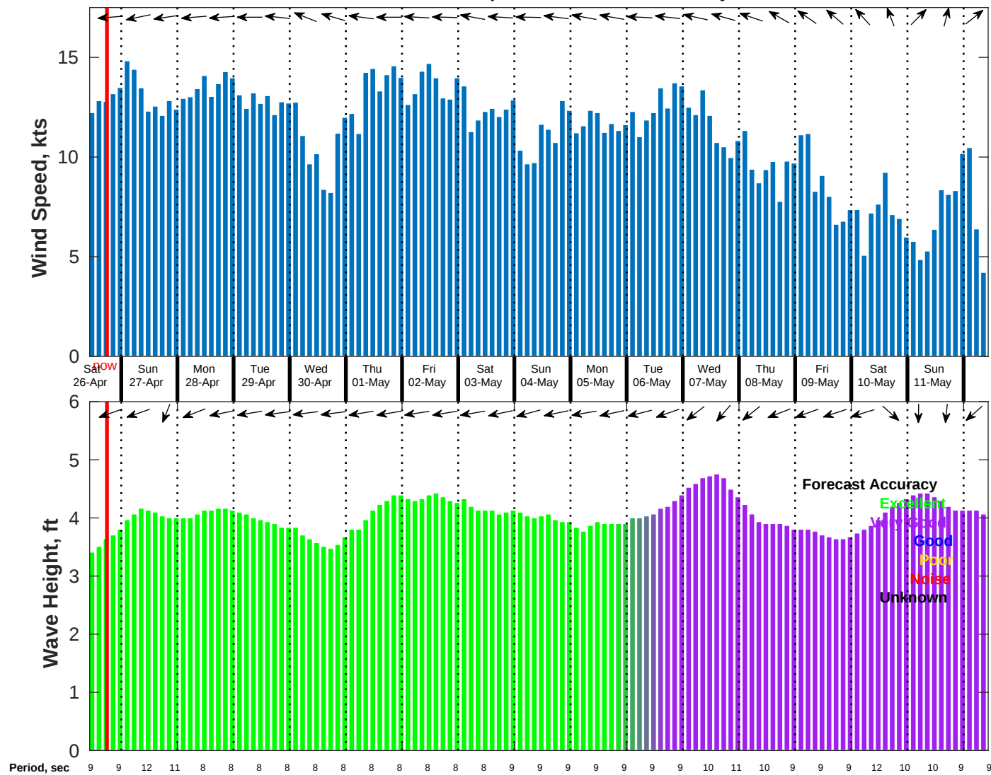
Wind & Wave Forecast for NDBC 52211 from 25-Apr-2025 10:00:00 to 11-May-2025 10:00:00
