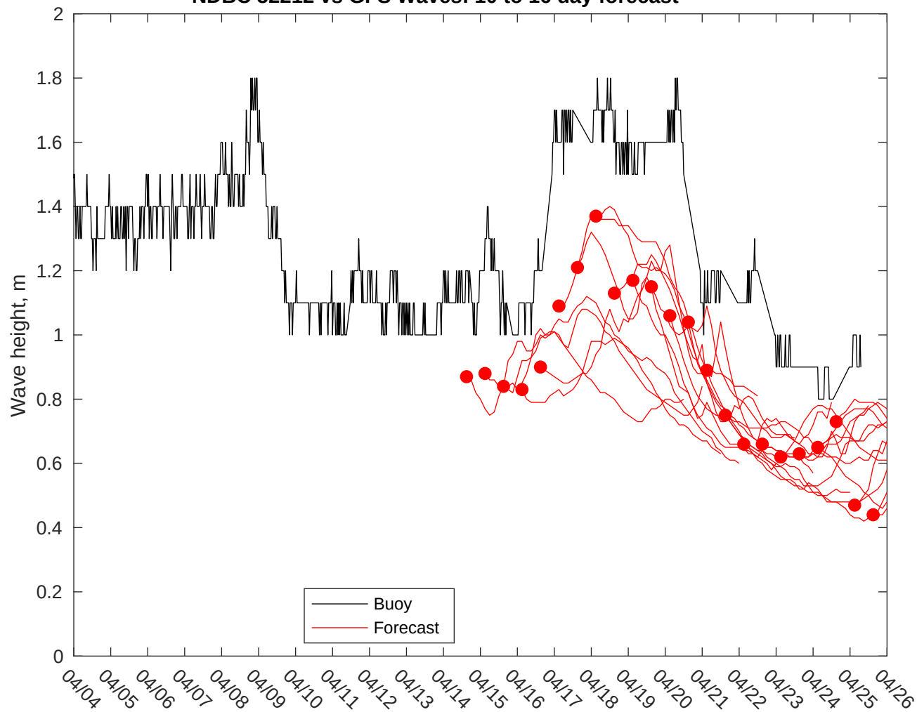
NDBC 52212 vs GFS Waves: 10 to 16 day forecast
