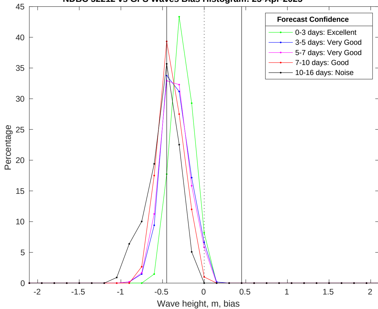
NDBC 52212 vs GFS Waves Bias Histogram: 25-Apr-2025
