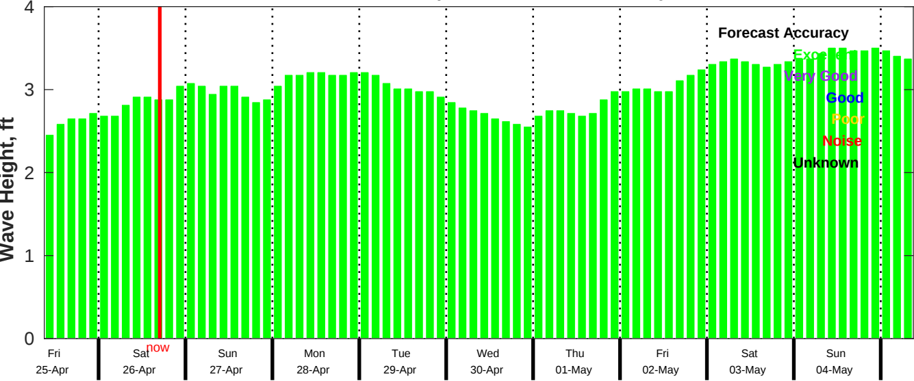
CMEMS Wave Forecast for NDBC 52212 from 24-Apr-2025 09:00:00 to 04-May-2025 09:00:00
