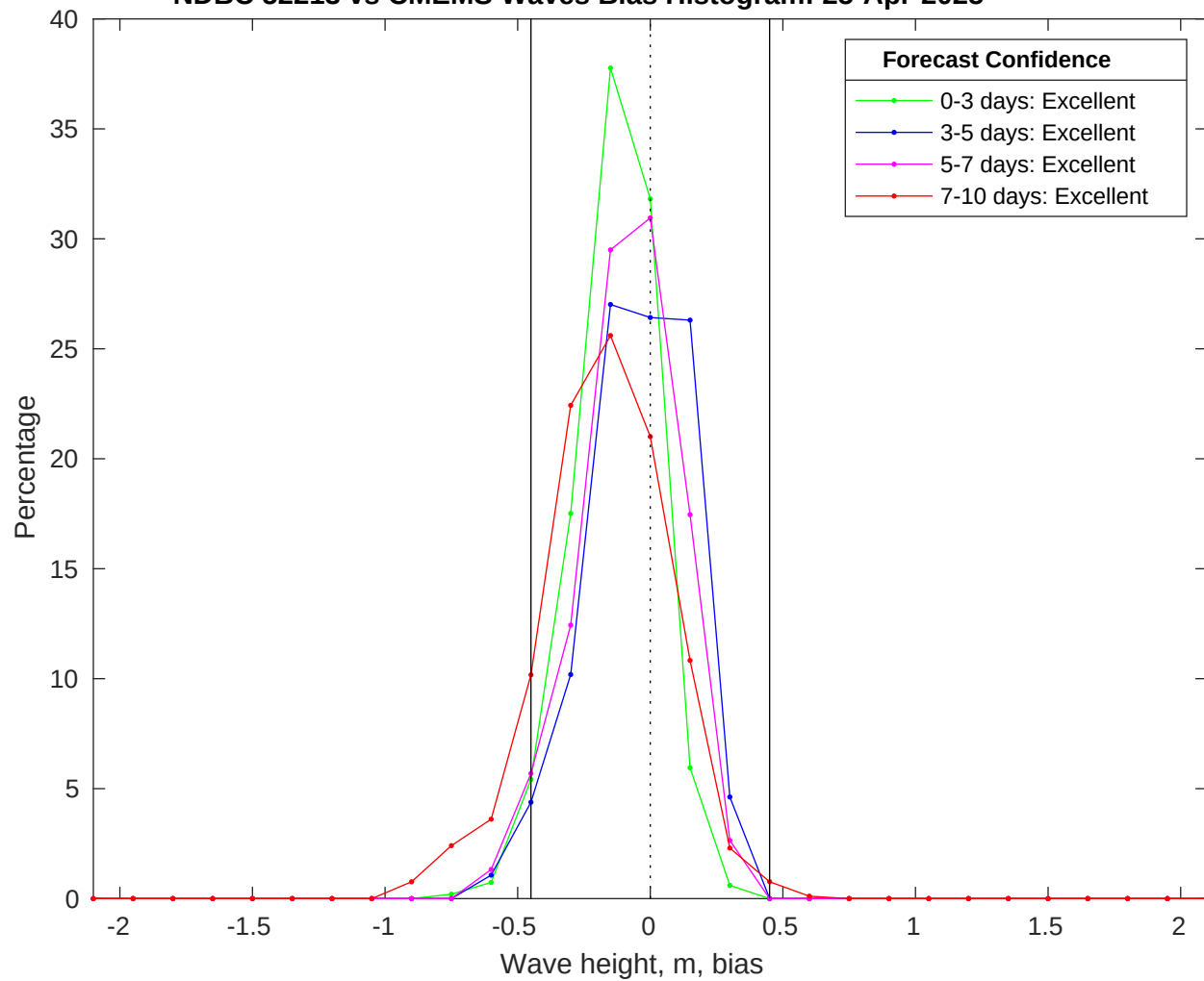
NDBC 52213 vs CMEMS Waves Bias Histogram: 25-Apr-2025
