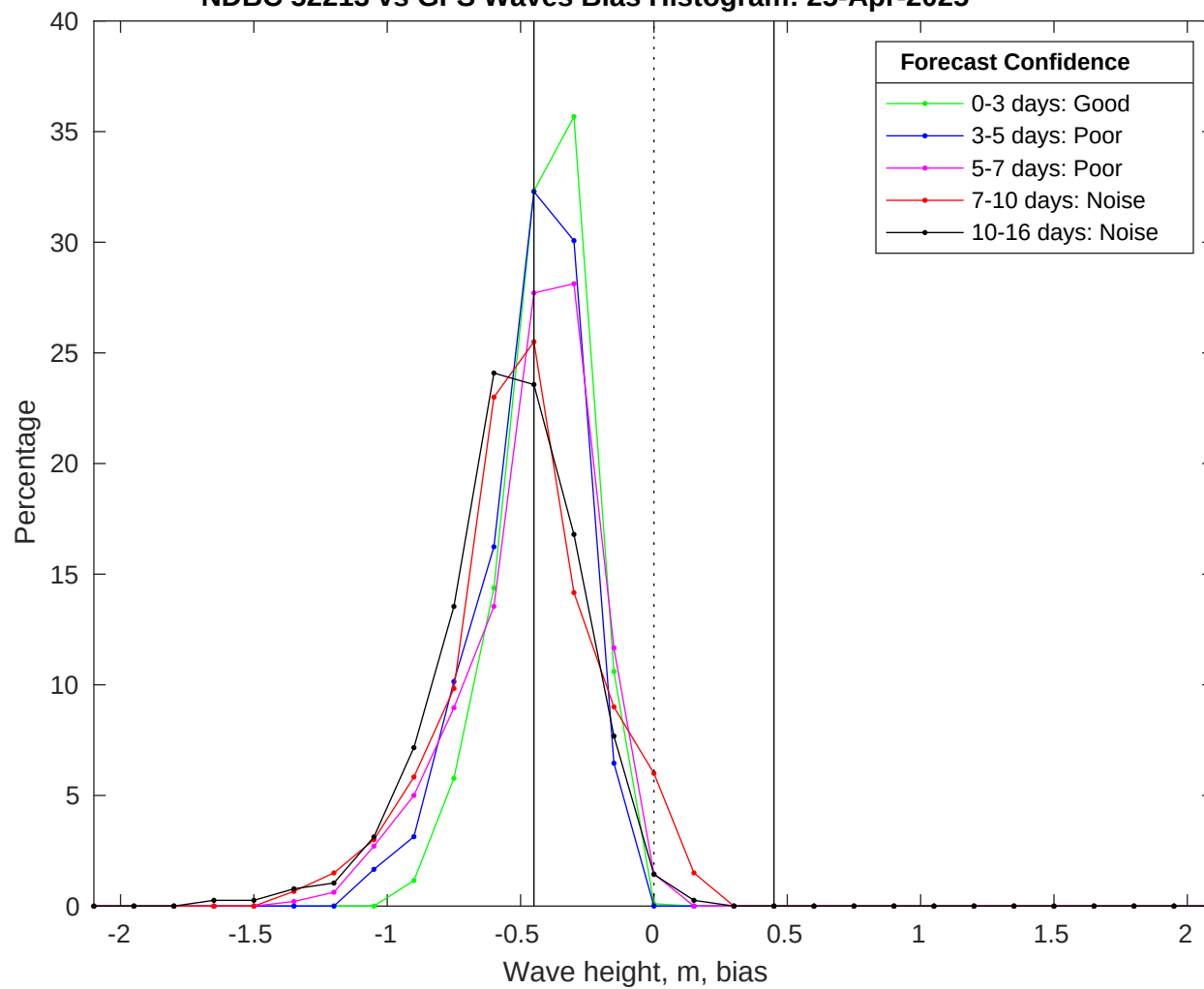
NDBC 52213 vs GFS Waves Bias Histogram: 25-Apr-2025
