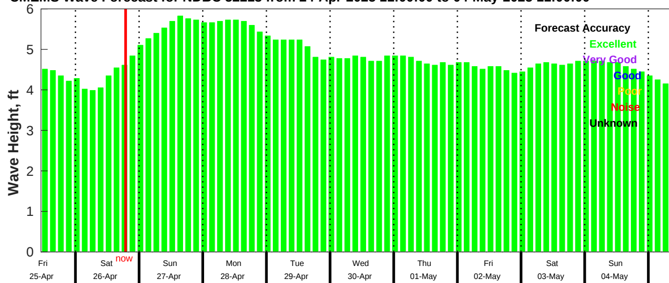
CMEMS Wave Forecast for NDBC 52213 from 24-Apr-2025 11:00:00 to 04-May-2025 11:00:00
