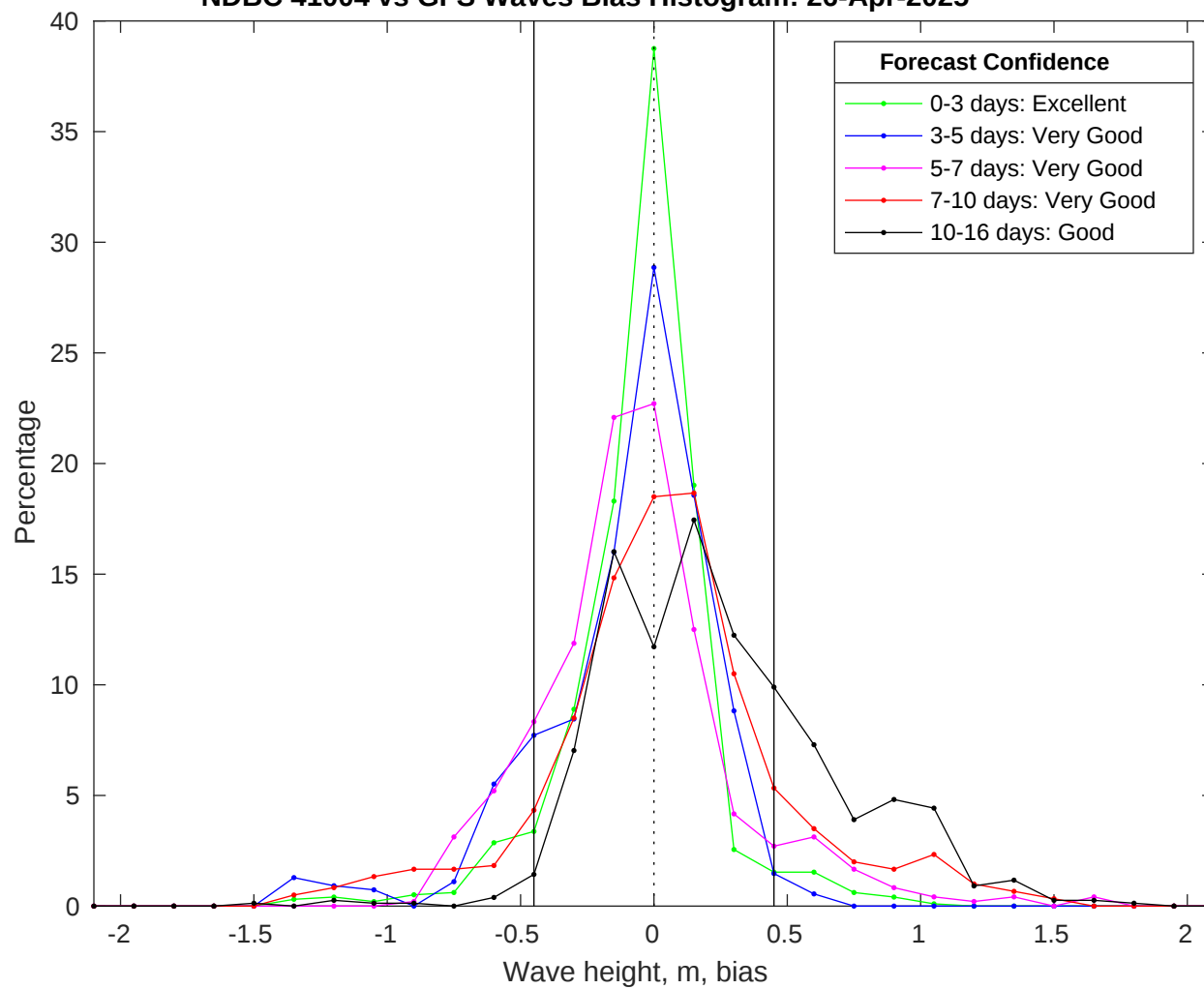
NDBC 41004 vs GFS Waves Bias Histogram: 26-Apr-2025
