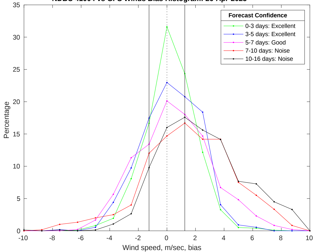
NDBC 41004 vs GFS Winds Bias Histogram: 26-Apr-2025
