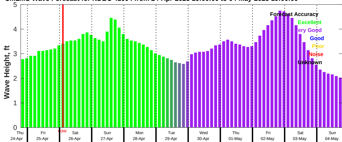
CMEMS Wave Forecast for NDBC 41004 from 24-Apr-2025 19:00:00 to 04-May-2025 19:00:00
