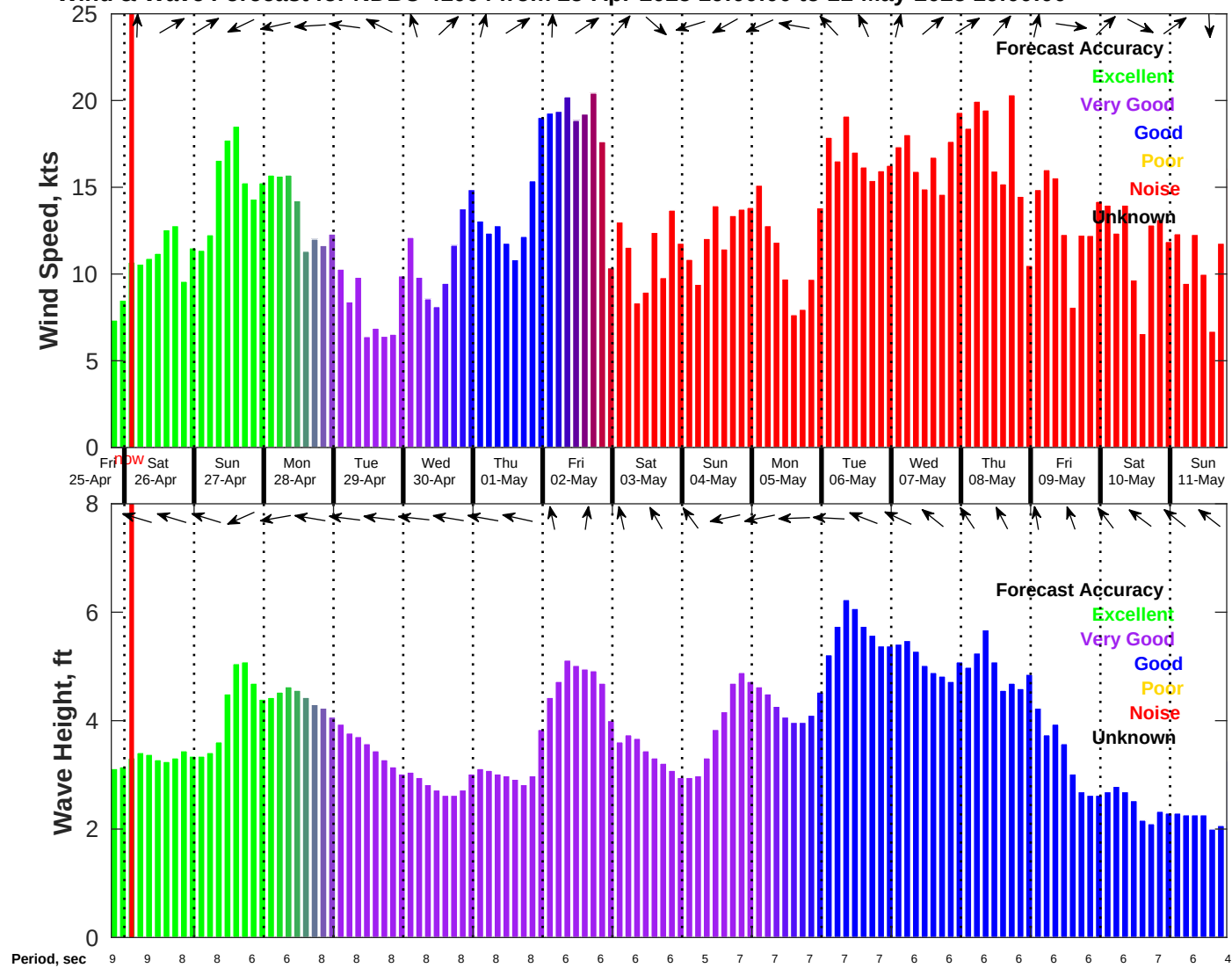
Wind & Wave Forecast for NDBC 41004 from 25-Apr-2025 19:00:00 to 11-May-2025 19:00:00
