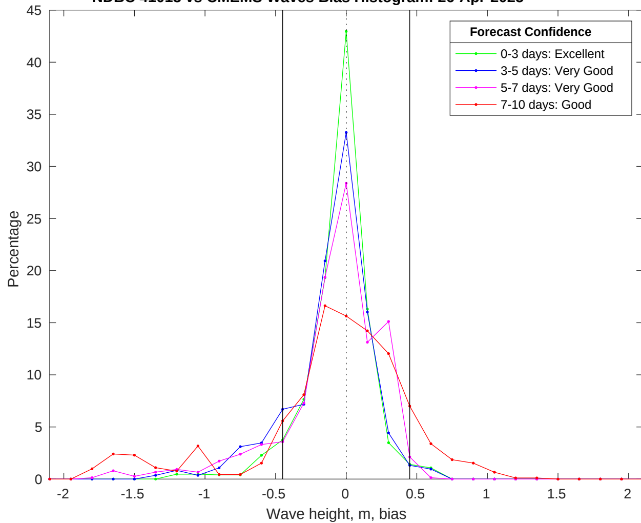
NDBC 41013 vs CMEMS Waves Bias Histogram: 26-Apr-2025
