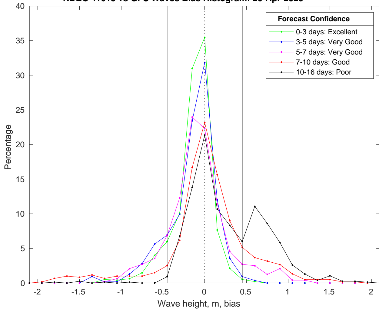
NDBC 41013 vs GFS Waves Bias Histogram: 26-Apr-2025
