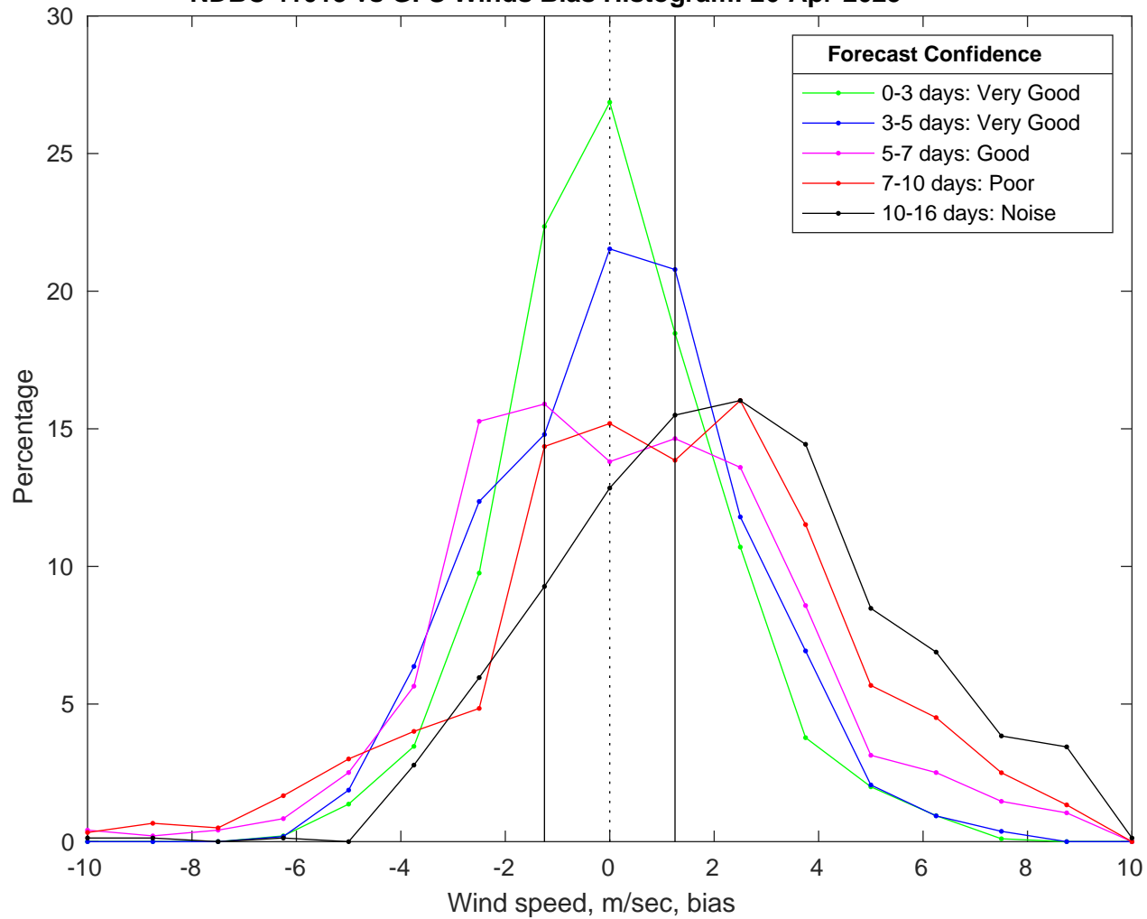
NDBC 41013 vs GFS Winds Bias Histogram: 26-Apr-2025
