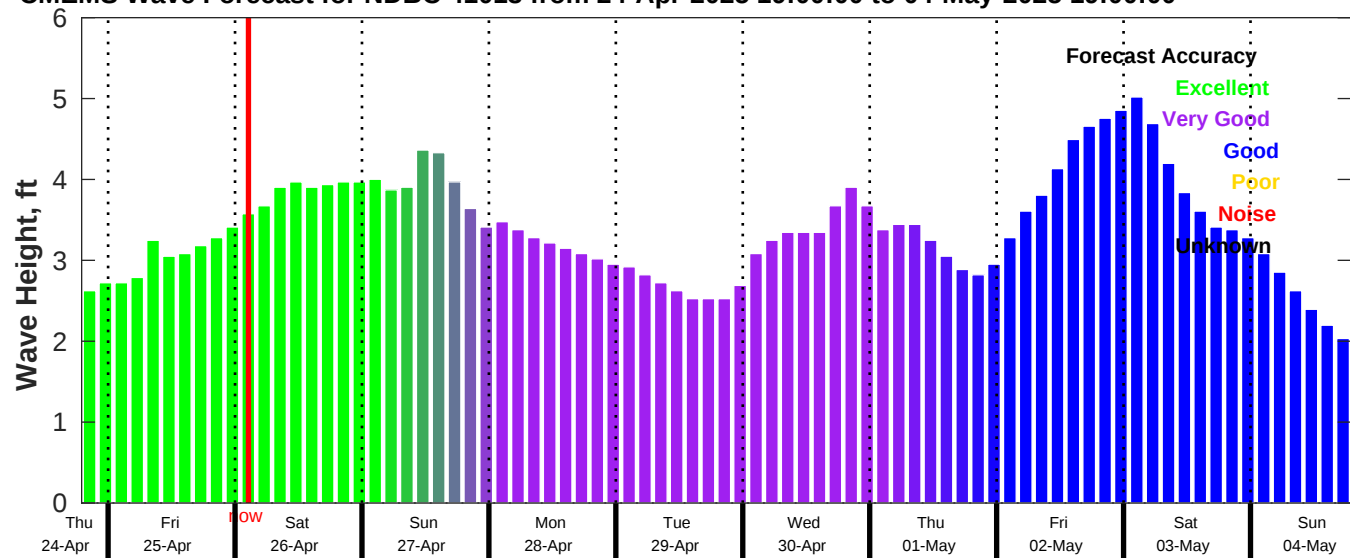
CMEMS Wave Forecast for NDBC 41013 from 24-Apr-2025 19:00:00 to 04-May-2025 19:00:00
