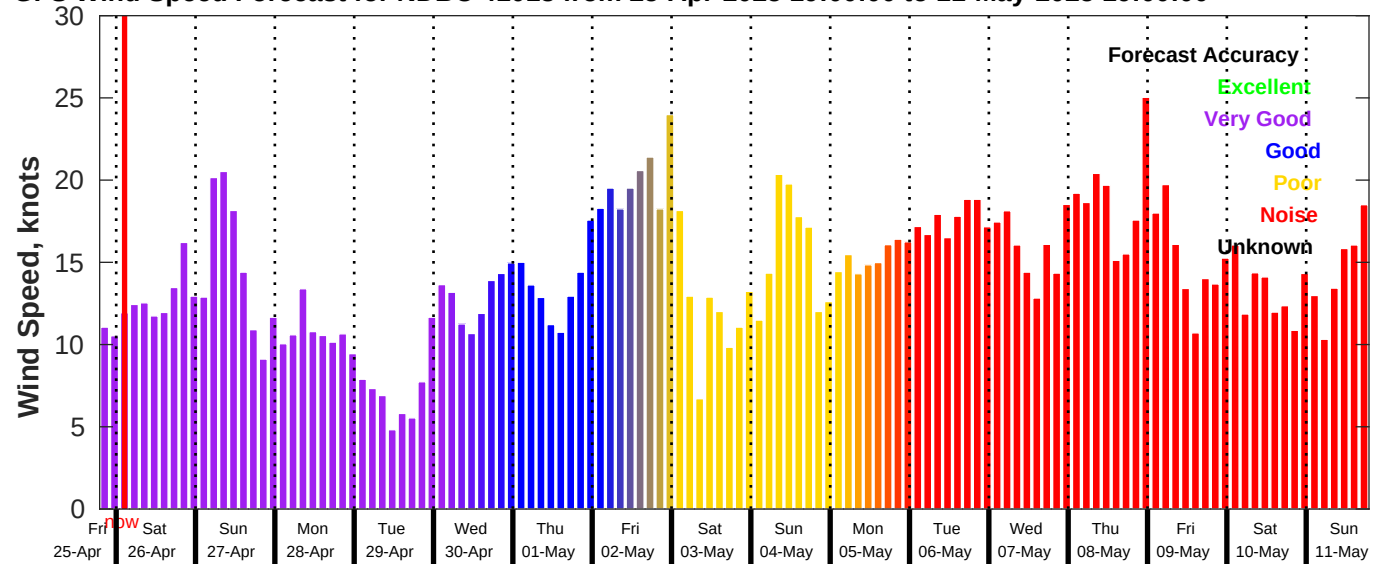
GFS Wind Speed Forecast for NDBC 41013 from 25-Apr-2025 19:00:00 to 11-May-2025 19:00:00
