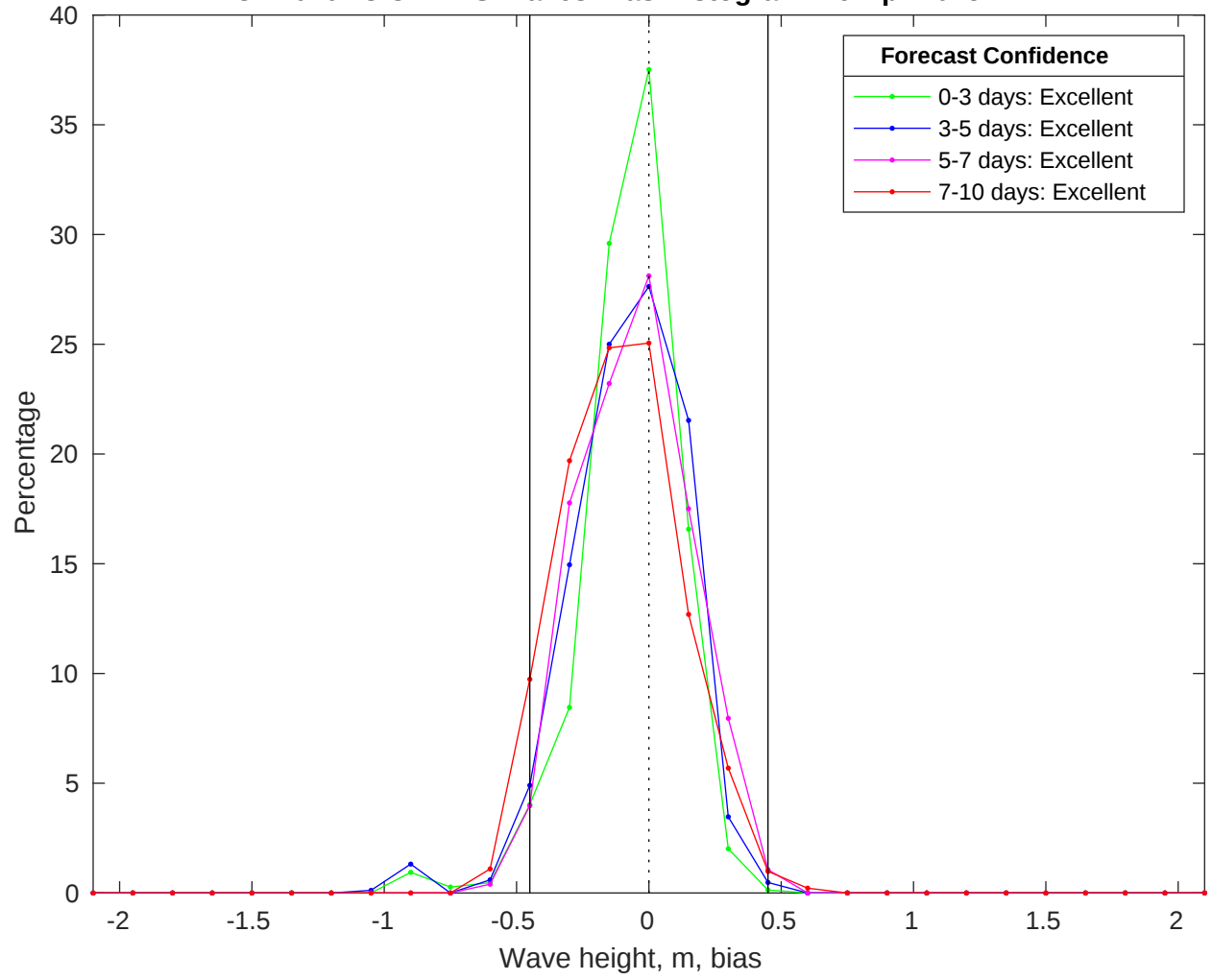
NDBC 41040 vs CMEMS Waves Bias Histogram: 26-Apr-2025
