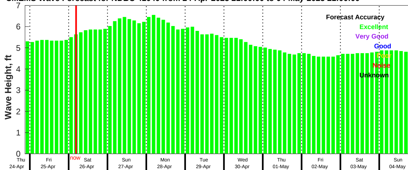
CMEMS Wave Forecast for NDBC 41040 from 24-Apr-2025 21:00:00 to 04-May-2025 21:00:00
