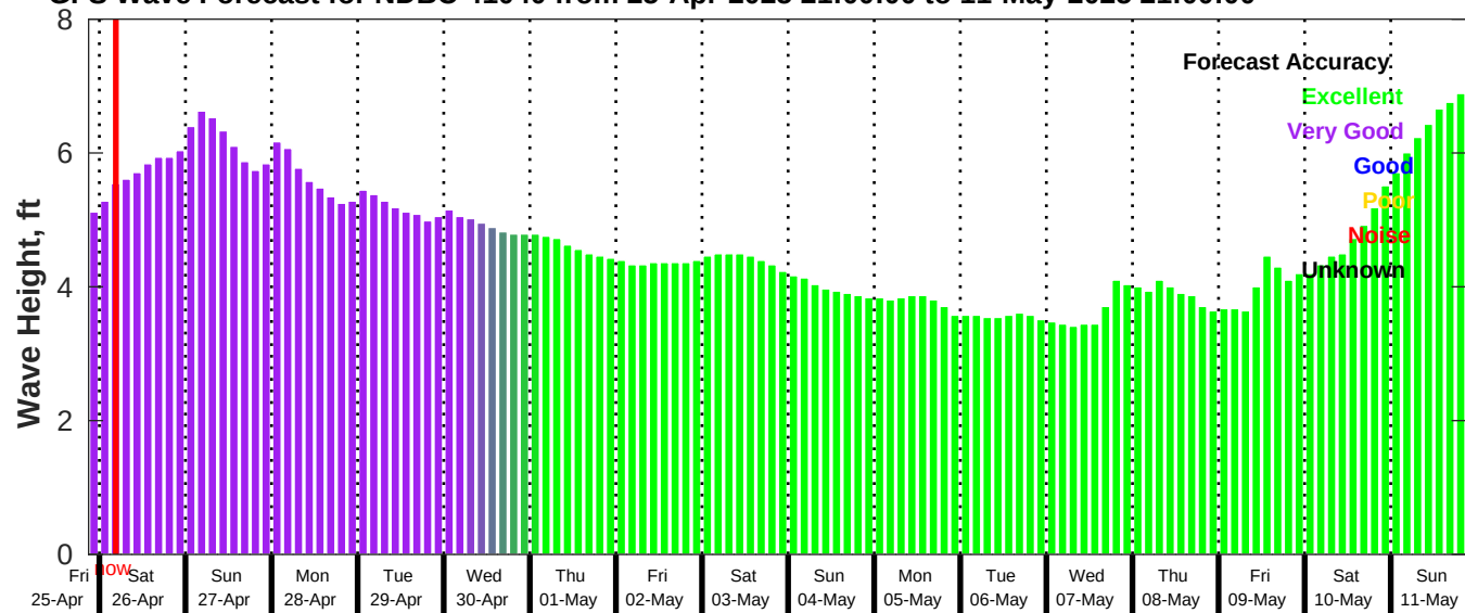
GFS Wave Forecast for NDBC 41040 from 25-Apr-2025 21:00:00 to 11-May-2025 21:00:00
