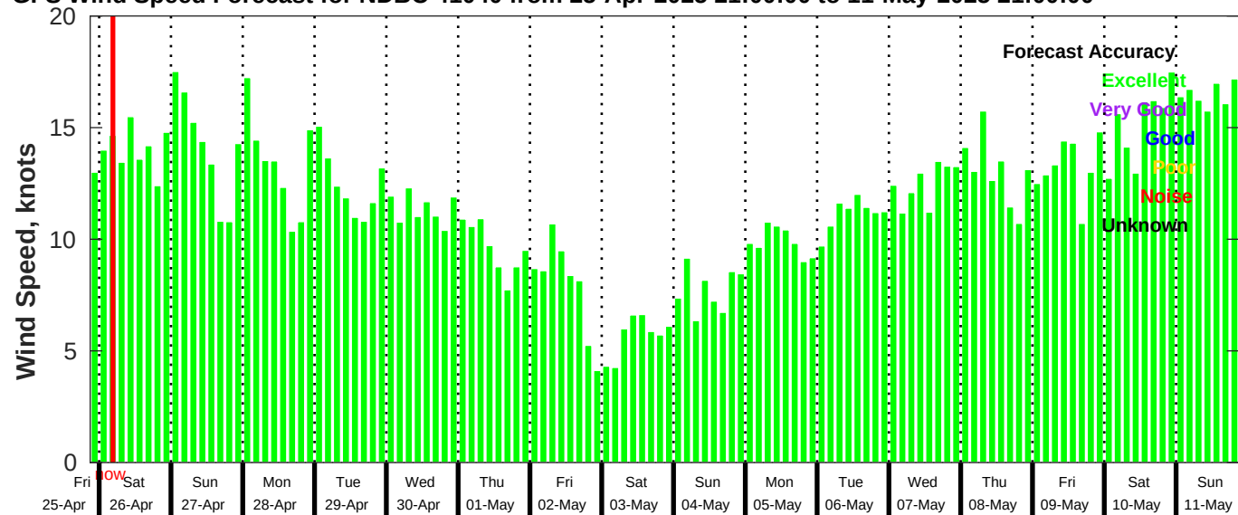
GFS Wind Speed Forecast for NDBC 41040 from 25-Apr-2025 21:00:00 to 11-May-2025 21:00:00
