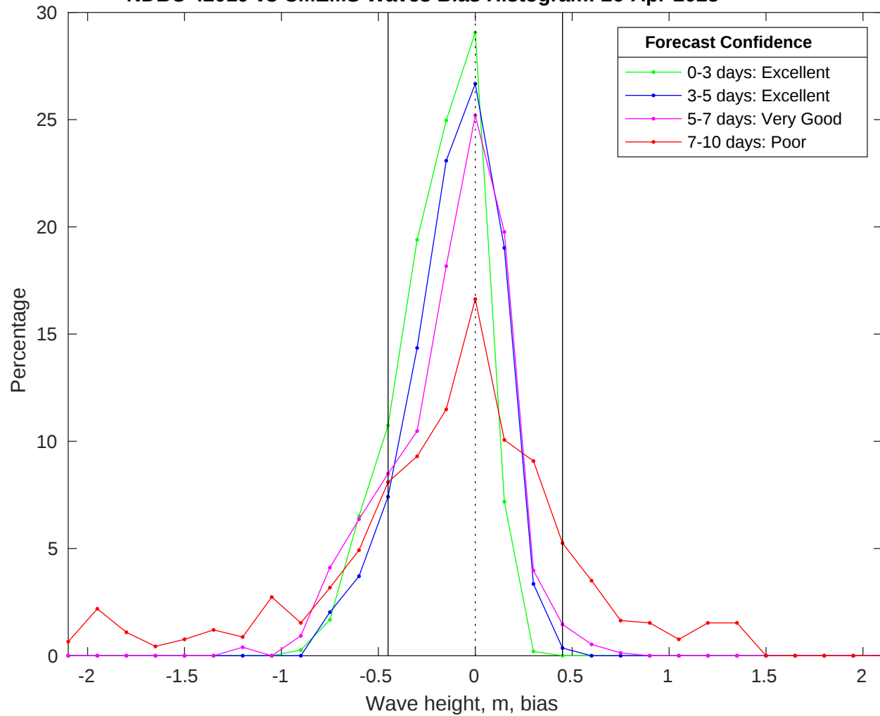
NDBC 42019 vs CMEMS Waves Bias Histogram: 26-Apr-2025
