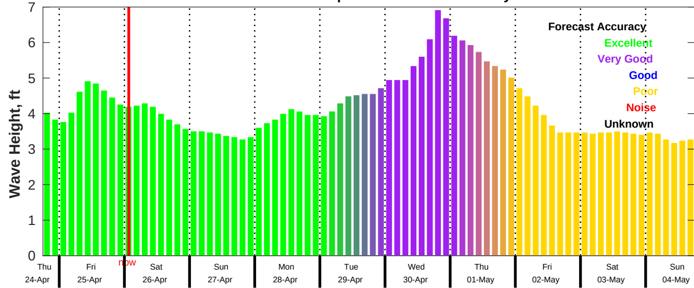
CMEMS Wave Forecast for NDBC 42019 from 24-Apr-2025 18:00:00 to 04-May-2025 18:00:00
